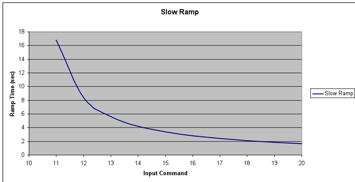
Figure 8.2: Slow Ramp
