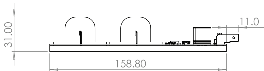
FIGURE 6. Side Mechanical view and dimensions
