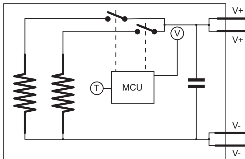
FIGURE 1. Simplified Block Diagram of Shunt Regulator Assembly
