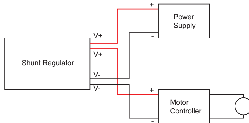
FIGURE 2. Connection Diagram
