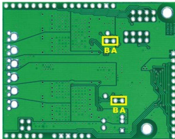
Cuttable traces on the dual VNH5019 motor driver shield for separately accessing ENA/DIAGA and ENB/DIAGB.
