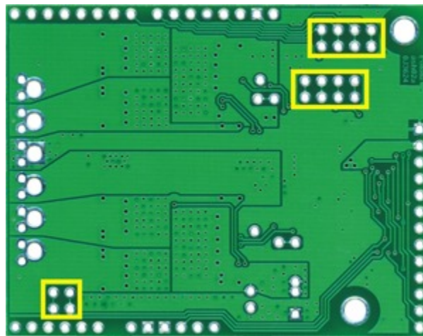
Cuttible traces on the dual VNH5019 motor driver shield for changing default Arduino pin mappings.
